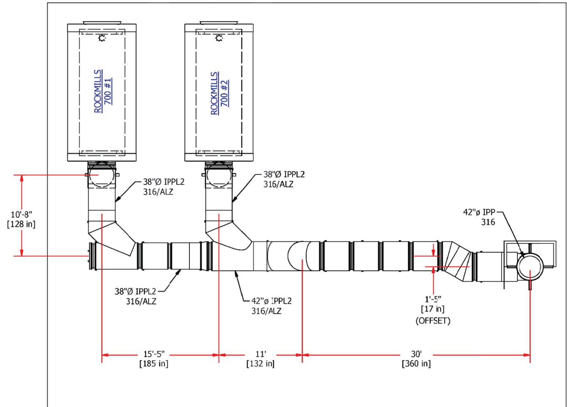
TOP VIEW
