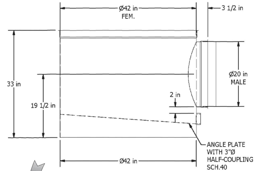
DETACHABLE BASE TEE DETAIL
