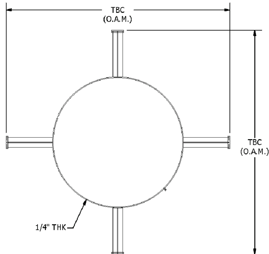
GUIDING SPACER/BUMPER DETAILS
